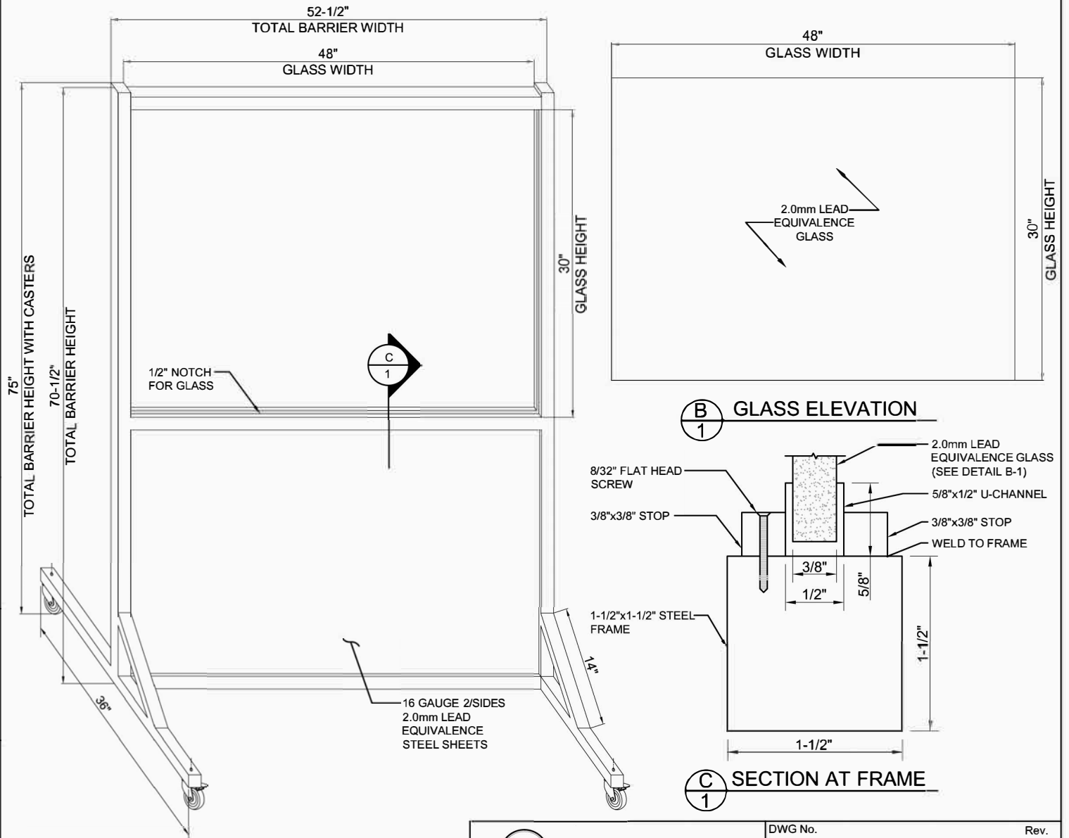
(A) BARRIER ELEVATION
