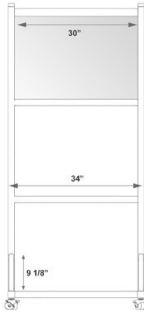
BACK VIEW
