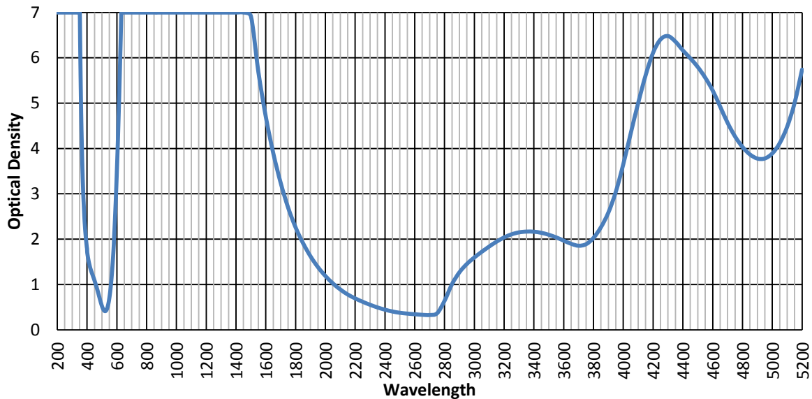
S8022F Optical Density
